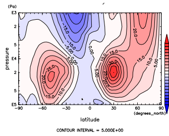
Figure 545: U at Feb. by NCEP
