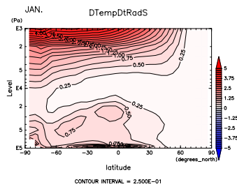
Figure 829: (\partial T/\partial t)_{sw} at Jan. by DCPAM
