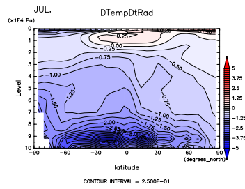
Figure 535: (\partial T/\partial t)_{SW+LW} at Jul. by DCPAM Figure 536: (\partial T/\partial t)_{SW+LW} at Aug. by DCPAM
