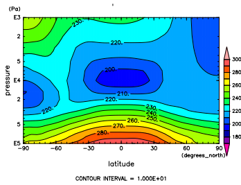
Figure 716: T at Nov. by NCEP
