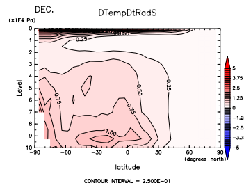
Figure 516: (\partial T / \partial t)_{sw} at Dec. by DCPAM
