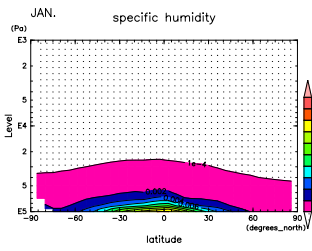
Figure 721: q at Jan. by DCPAM
