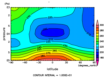
Figure 719: T at Dec. by NCEP
