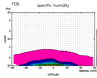
Figure 724: q at Feb. by DCPAM
