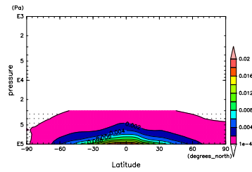
Figure 730: q at Apr. by DCPAM
