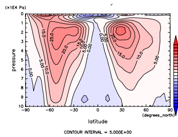
Figure 227: U at Apr. by NCEP
