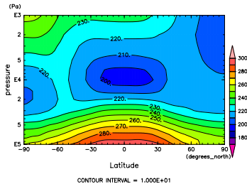
Figure 715: T at Nov. by DCPAM
