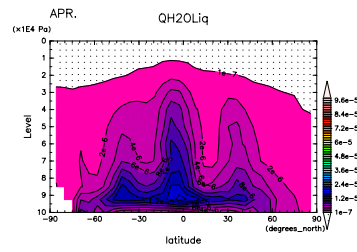
Figure 472: q_l at Apr. by DCPAM
