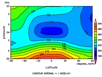
Figure 718: T at Dec. by DCPAM
