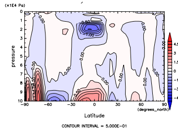
Figure 313: V at Sep. by DCPAM
