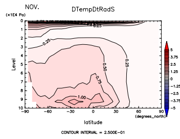
Figure 515: (\partial T / \partial t)_{sw} at Nov. by DCPAM
