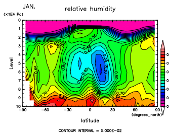
Figure 433: RH at Jan. by DCPAM
