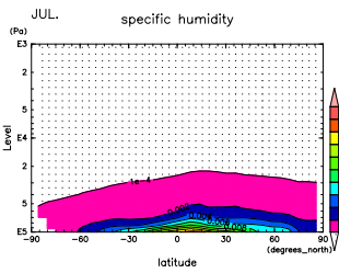
Figure 739: q at Jul. by DCPAM
