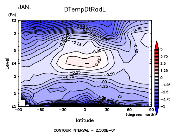
Figure 841: (\partial T/\partial t)_{LW} at Jan. by DCPAM
