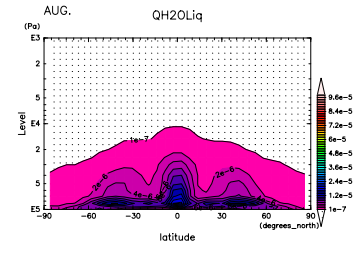
Figure 800: q_l at Aug. by DCPAM
