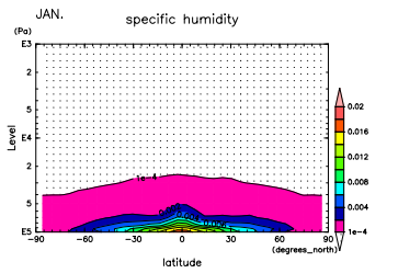
Figure 721: q at Jan. by DCPAM
