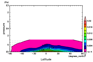
Figure 736: q at Jun. by DCPAM
