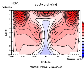
Figure 247: U at Nov. by DCPAM
