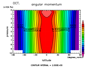
Figure 280: ANGMOM at Oct. by DCPAM
