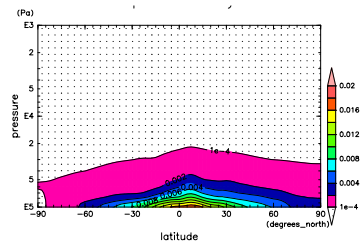
Figure 737: q at Jun. by NCEP
