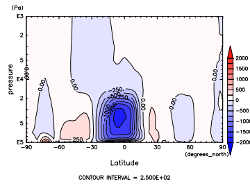
Figure 670: MSF at Aug. by DCPAM
