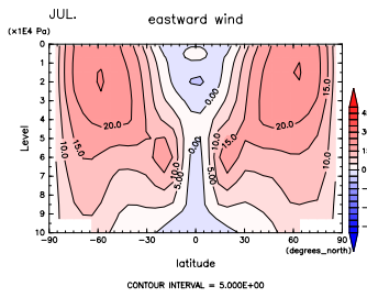
Figure 235: U at Jul. by DCPAM
