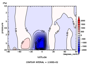
Figure 668: MSF at Jul. by NCEP
