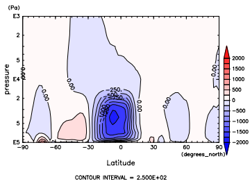
Figure 667: MSF at Jul. by DCPAM
