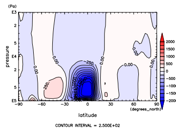
Figure 671: MSF at Aug. by NCEP
