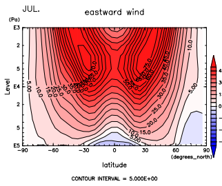
Figure 559: U at Jul. by DCPAM
