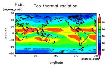
Figure 122: OLR at Jan. by NCEP Figure 125: OLR at Feb. by NCEP
