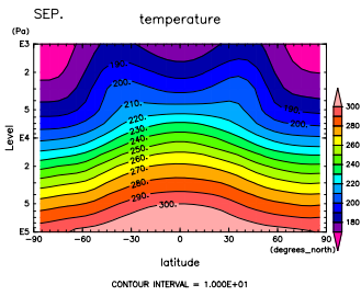
Figure 709: T at Sep. by DCPAM
