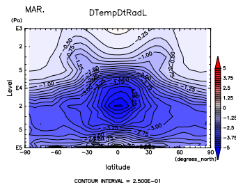
Figure 843: (\partial T/\partial t)_{LW} at Mar. by DCPAM by Figure 844: (\partial T/\partial t)_{LW} at Apr. by DCPAM
