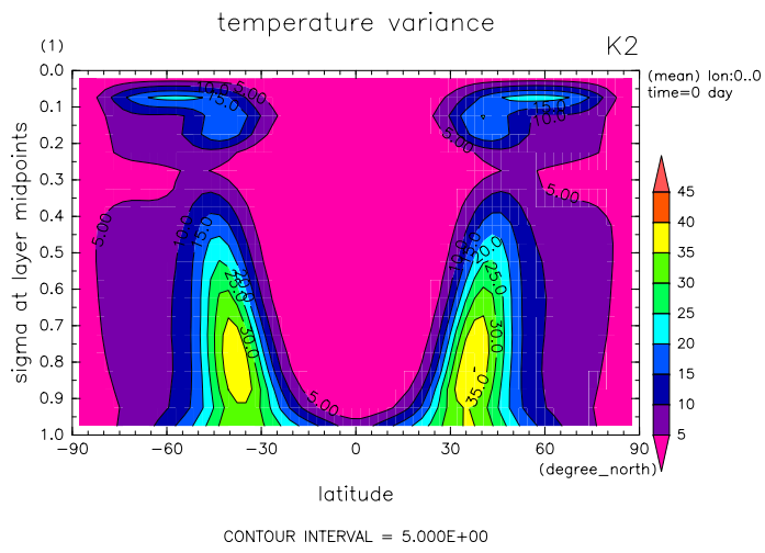
Figure 3: Zonal mean zonal eddy temperature squared by dpam
