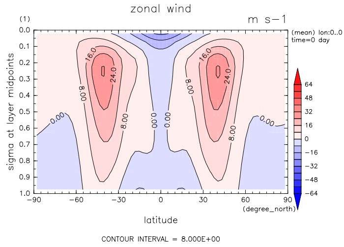
Figure 1: Zonal mean zonal wind by dcpan
