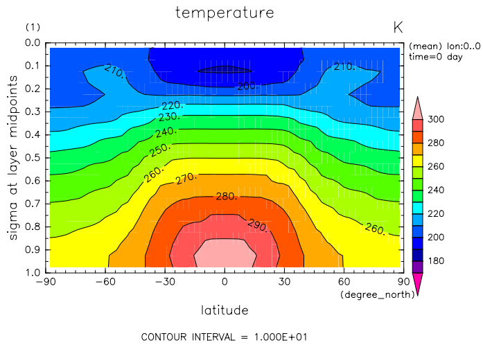
Figure 2: Zonal mean temperature by dpam
