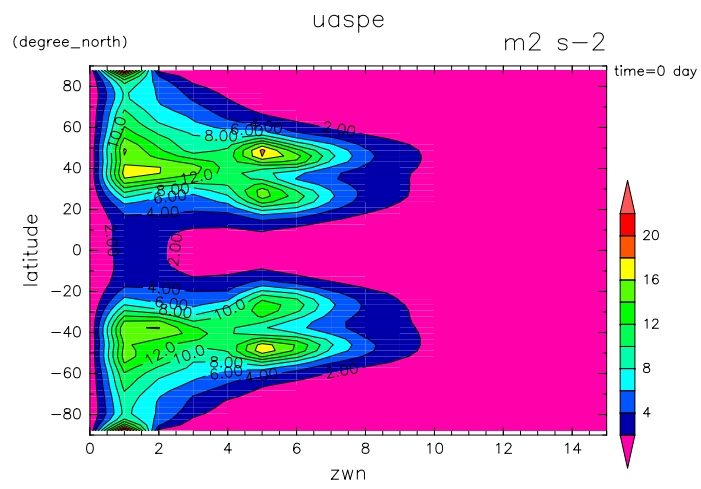
Figure 5: Spectrum of zonal wind by depam
