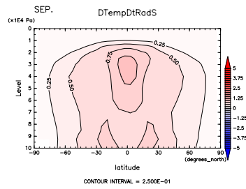
Figure 513: (\partial T/\partial t)_{sw} at Sep. by DCPAM
