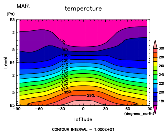
Figure 691: T at Mar. by DCPAM
