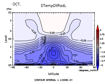
Figure 849: (\partial T / \partial t)_{LW} at Sep. by DCPAM by Figure 850: (\partial T / \partial t)_{LW} at Oct. by DCPAM
