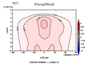
Figure 514: (\partial T/\partial t)_{sw} at Oct. by DCPAM
