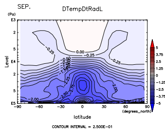
Figure 849: (\partial T / \partial t)_{LW} at Sep. by DCPAM by Figure 850: (\partial T / \partial t)_{LW} at Oct. by DCPAM
