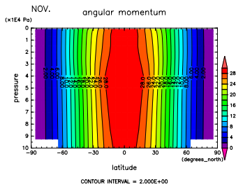
Figure 283: ANGMOM at Nov. by DCPAM by Figure 286: ANGMOM at Dec. by DCPAM
