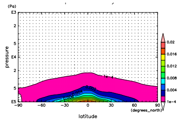
Figure 731: q at Apr. by NCEP
