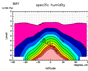
Figure 409: q at May by DCPAM
