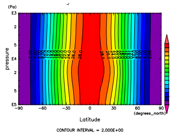
Figure 610: ANG MOM at Dec. by DCPAM
