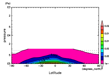
Figure 724: q at Feb. by DCPAM
