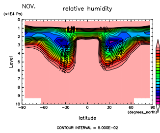
Figure 463: RH at Nov. by DCPAM
