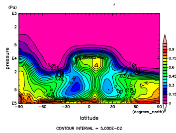
Figure 785: RH at Oct. by NCEP
