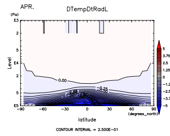
Figure 844: (\partial T/\partial t)_{LW} at Apr. by DCPAM
