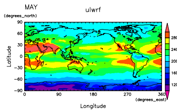
Figure 133: OLR at May by DCPAM
