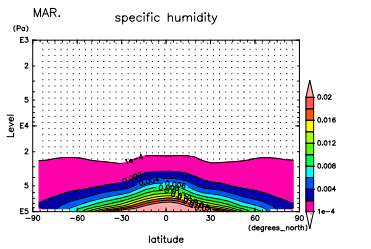
Figure 727: q at Mar. by DCPAM
