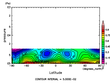
Figure 784: RH at Oct. by DCPAM
