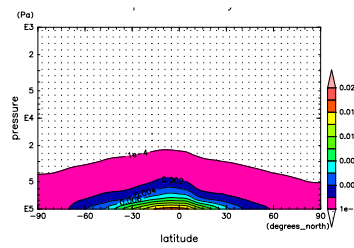
Figure 725: q at Feb. by NCEP
