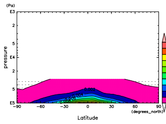
Figure 751: q at Nov. by DCPAM
