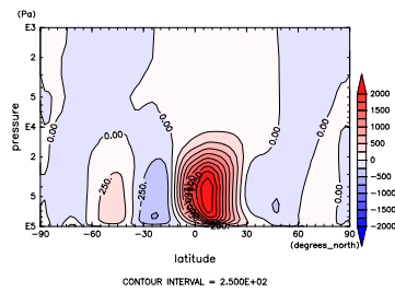
Figure 650: MSF at Jan. by NCEP Figure 653: MSF at Feb. by NCEP
