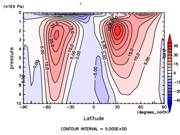
Figure 217: U at Jan. by DCPAM
