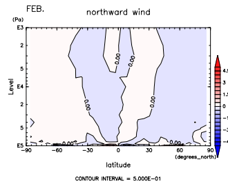
Figure 616: V at Feb. by DCPAM
