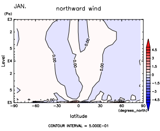
Figure 613: V at Jan. by DCPAM
