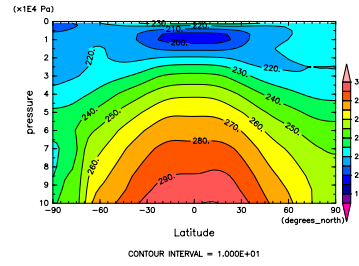
Figure 370: T at Apr. by DCPAM
