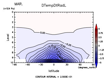
Figure 519: (\partial T/\partial t)_{LW} at Mar. by DCPAM
