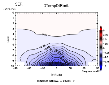
Figure 525: (\partial T/\partial t)_{LW} at Sep. by DCPAM
